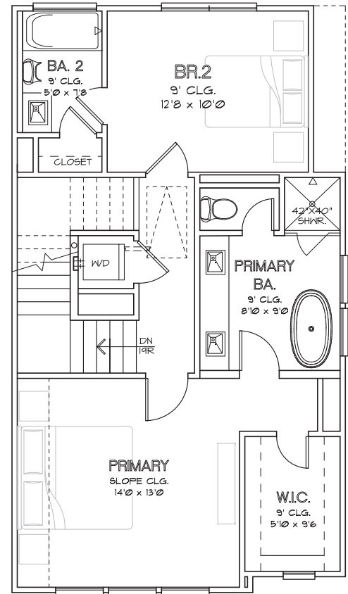
THIRD FLOOR
