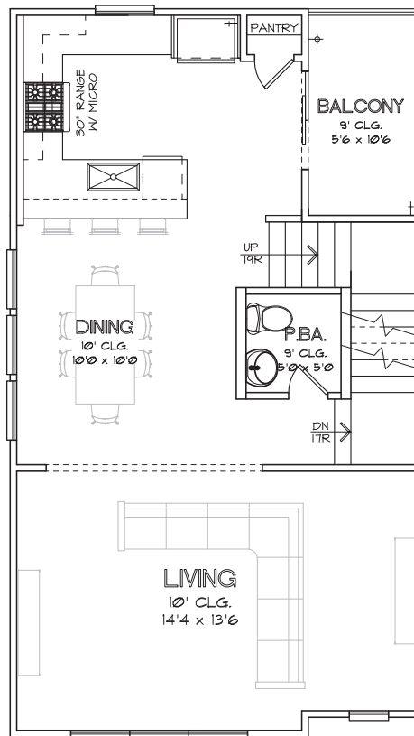
SECOND FLOOR
