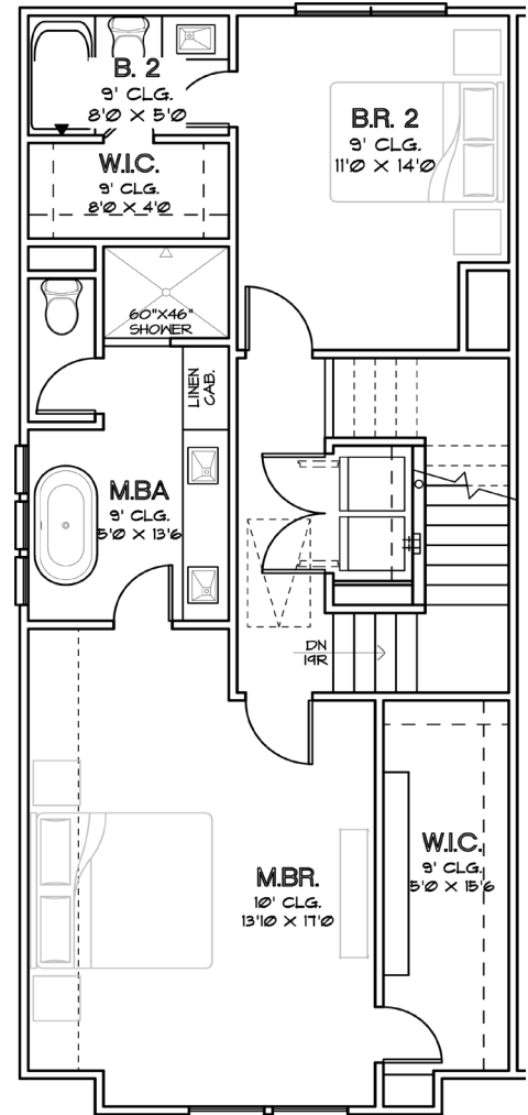
THIRD FLOOR
