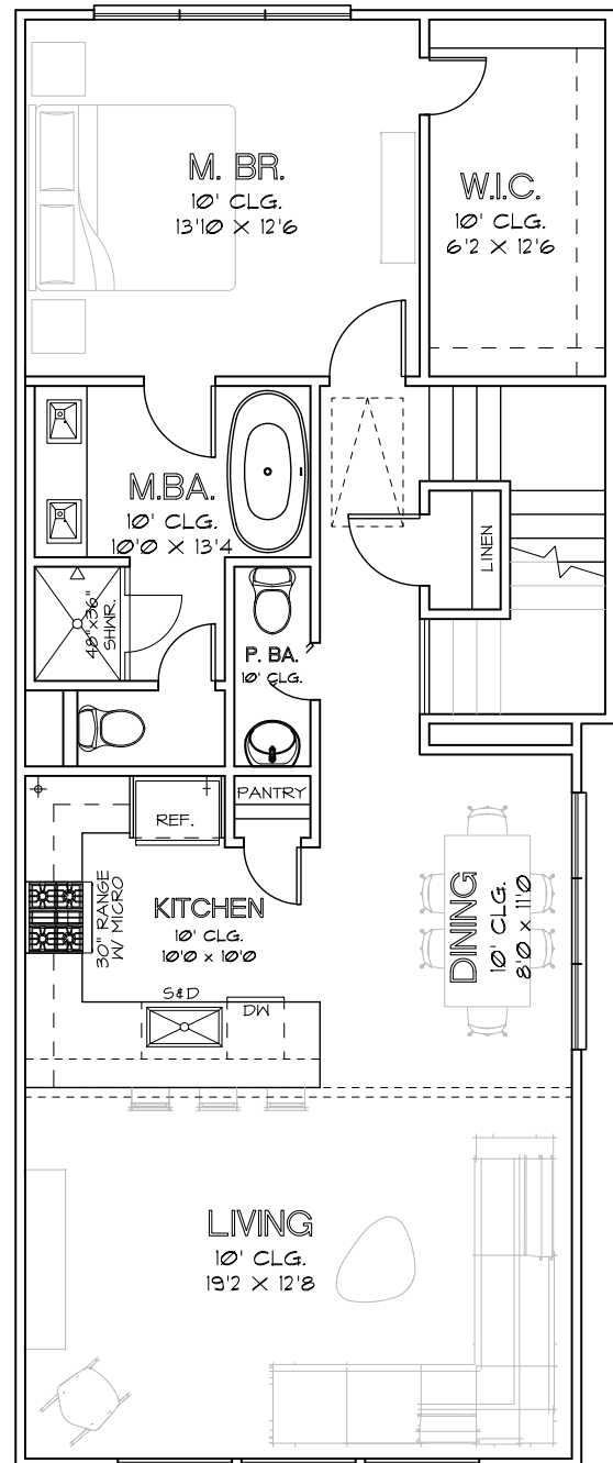
SECOND FLOOR
