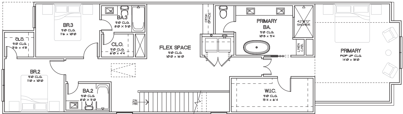
SECOND FLOOR
