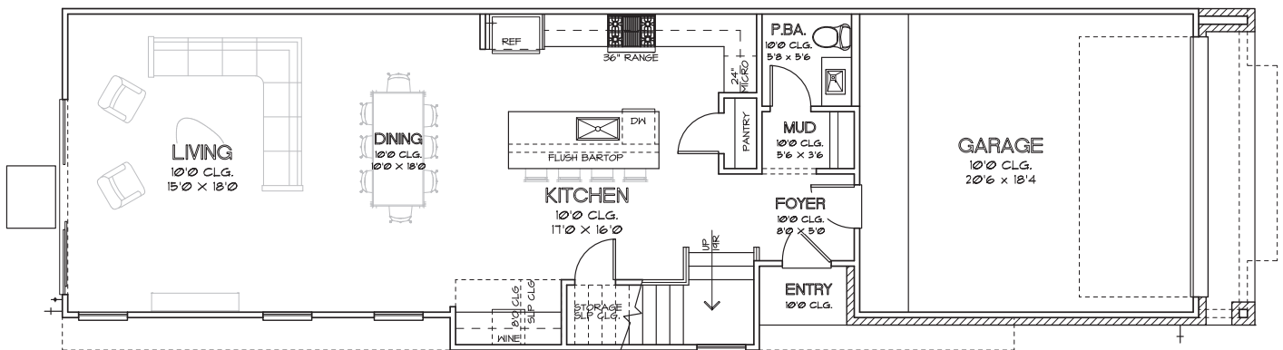
FIRST FLOOR
