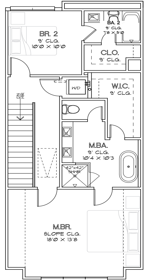
THIRD FLOOR
