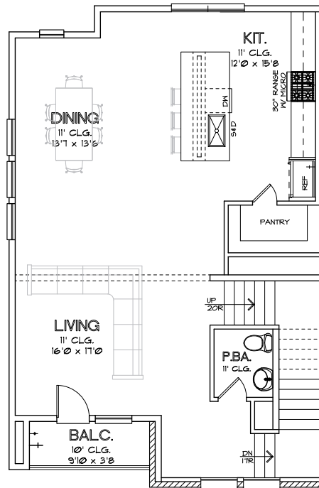
SECOND FLOOR
