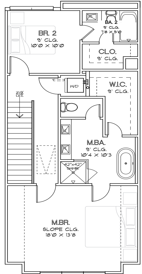
THIRD FLOOR
