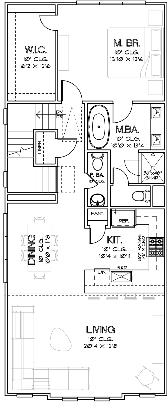
SECOND FLOOR
