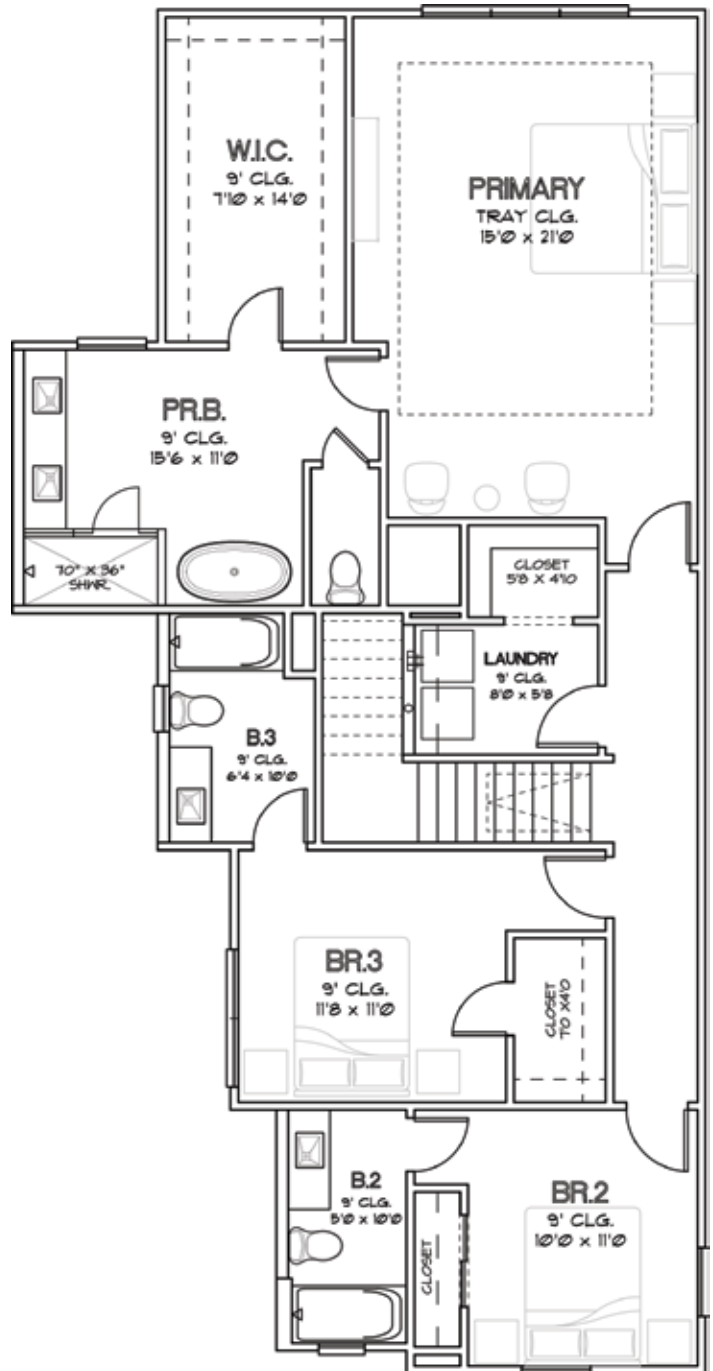
SECOND FLOOR
