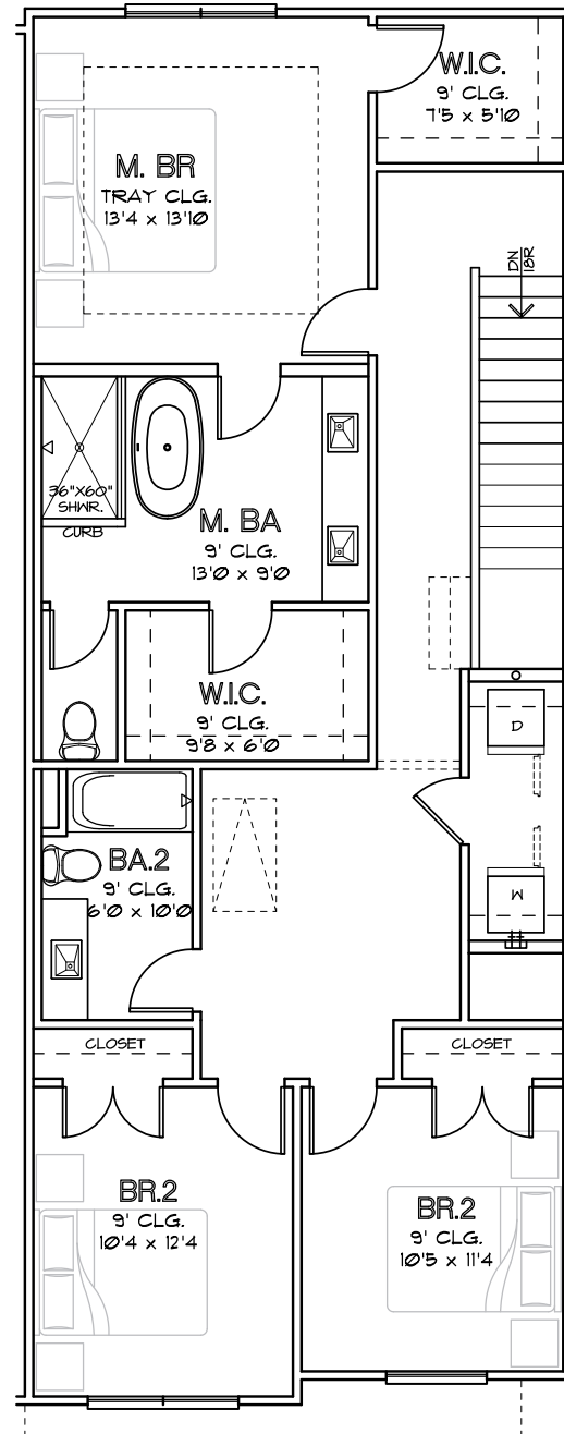
SECOND FLOOR
